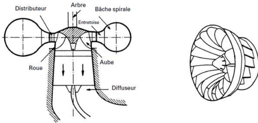
Figure.2-3 : Turbine Francis
