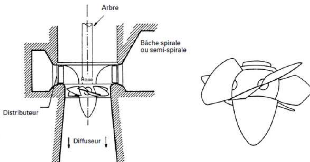
Figure.2-4 : Turbine Kaplan
